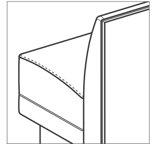
Applied 3/4" thick self edge plastic laminate or wood veneer back with welt
